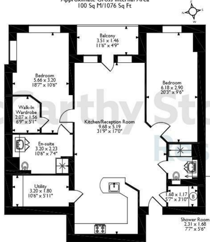
First Floor The position & size of doors, windows, appliances and other features are approximate only. © ehouse. Unauthorised reproduction prohibited. Drawing ref. dig/8657907/DST.
